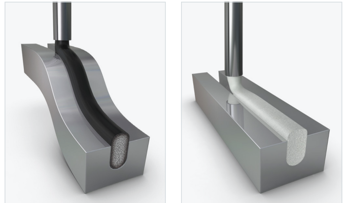
Sealing the 2D or 3D lamp housing groove with FERMAPOR K31 polyurethane foam or FERMASIL silicone foam
