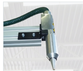
The optional plasma nozzle mounted on the back of the CNC Y-axis applies the plasma in parallel to the seal application onto plastic surfaces of the component in the same contour.
