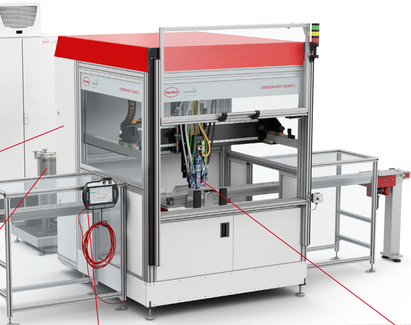
Alternative reference system of the SMART-L dosing cell with sliding table . Two shuttle tables operating in pendulum mode enable the parts to be processed on one level. This means that very short cycle times and continuous operation can be guaranteed.
