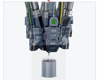
MK 825 PRO precision mixing head with high-pressure water rinsing
